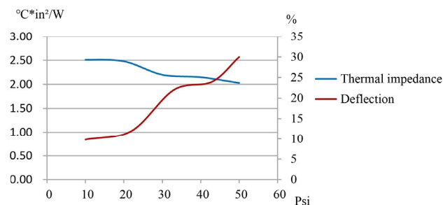
Pressure vs. Deflection SBC-3 - 3,0 mm
